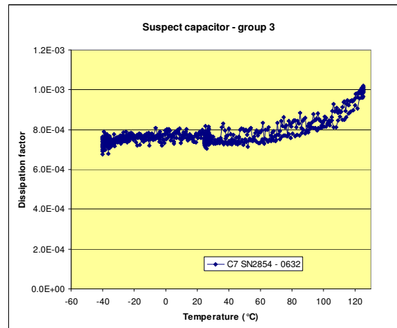
Figure 7 – Electrical comparison of Good vs. Counterfeit Capacitors
