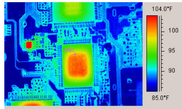
Figure 9 – Infrared Thermography
